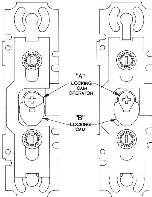
STANDARD LOCKING BACKPLATE FIGURE 1
