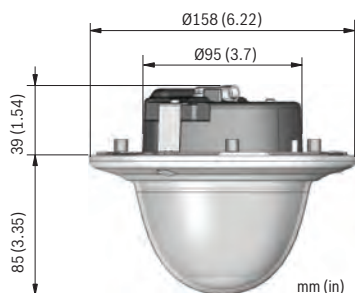
Flush-mount dimensions
