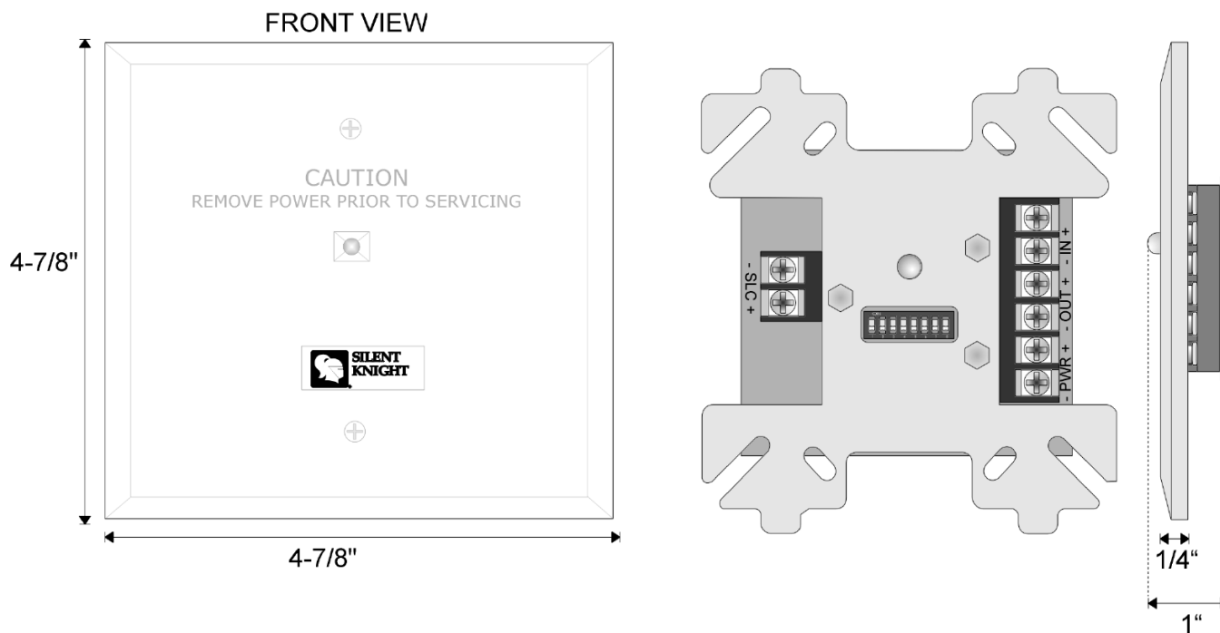
Model SD500-ANM Addressable Notification Module
