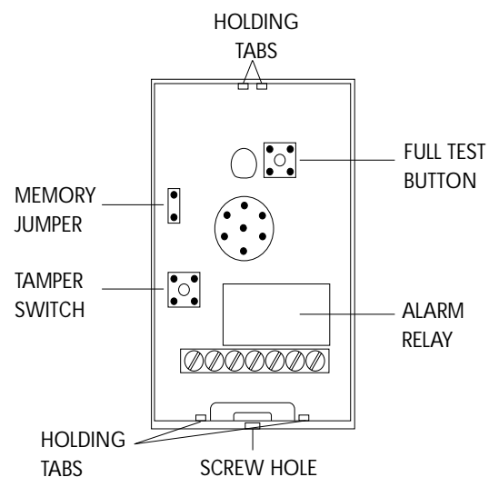
VITRON PCB - General View
