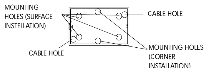
VITRON Mounting and Cable Holes
