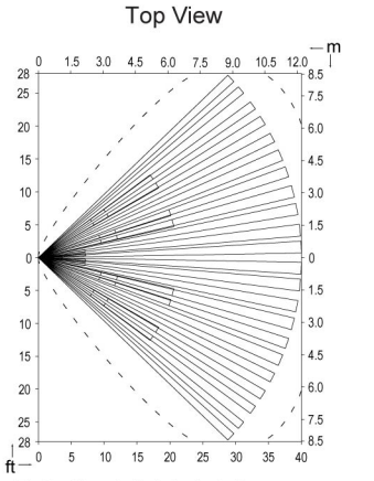
QT-40 & QT-40SL Main Lens: 40WAPET Wide Angle 40ft (12m) L X 56ft (17m) W
