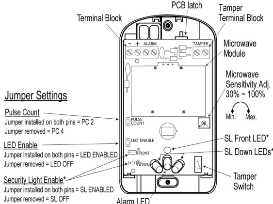
Fig. 2: PCB Layout
