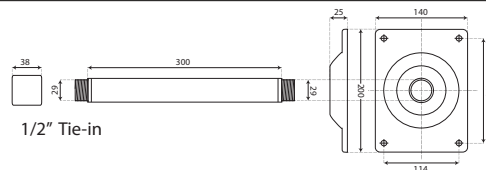
PTZPEND237X — LINE ART / MOUNTING CONFIG
