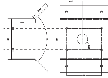
PTZCORNER12X — LINE ART / MOUNTING CONFIG
