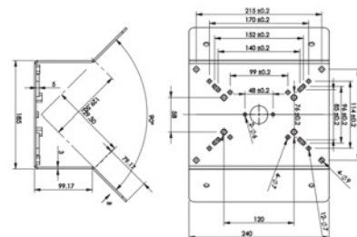
PTZCORNER237X — LINE ART / MOUNTING CONFIG
