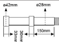
PTZPEND12X — LINE ART / MOUNTING CONFIG
