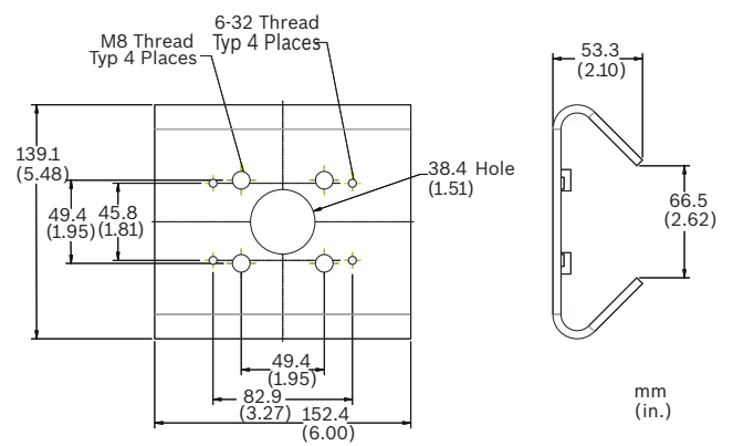
LTC 9213/01 Pole Mount Adapter dimensions
