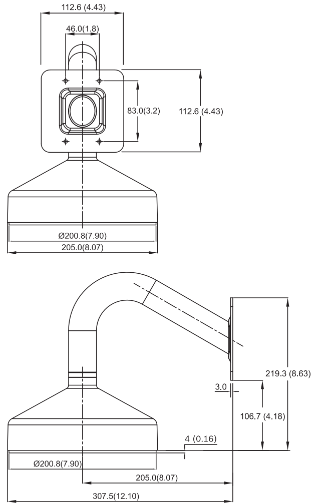
VDA-832FHD-WMT Wall mount dimensions
