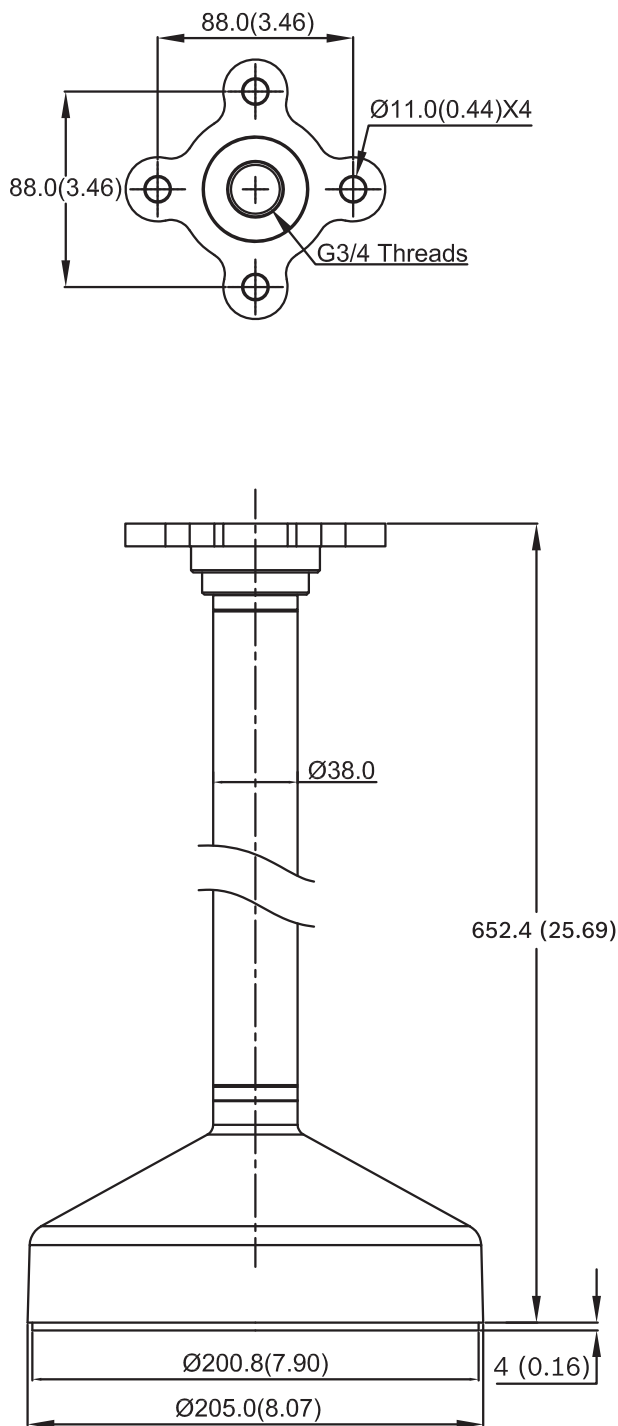
VDA-832FHD-PMT Pipe mount dimensions
