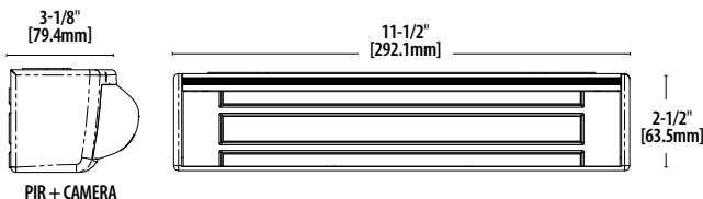
PIR + CAMERA
