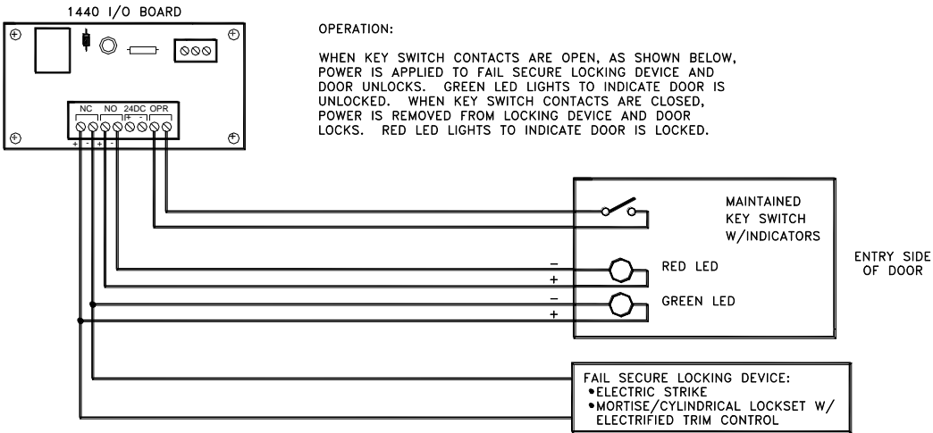
FIG. 2: WIRE SCHEME FOR A TYPICAL FAIL SECURE SYSTEM
