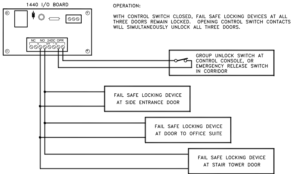
FIG. 3: WIRE SCHEME FOR SIMULTANEOUS CONTROL OF MULTIPLE DOORS
