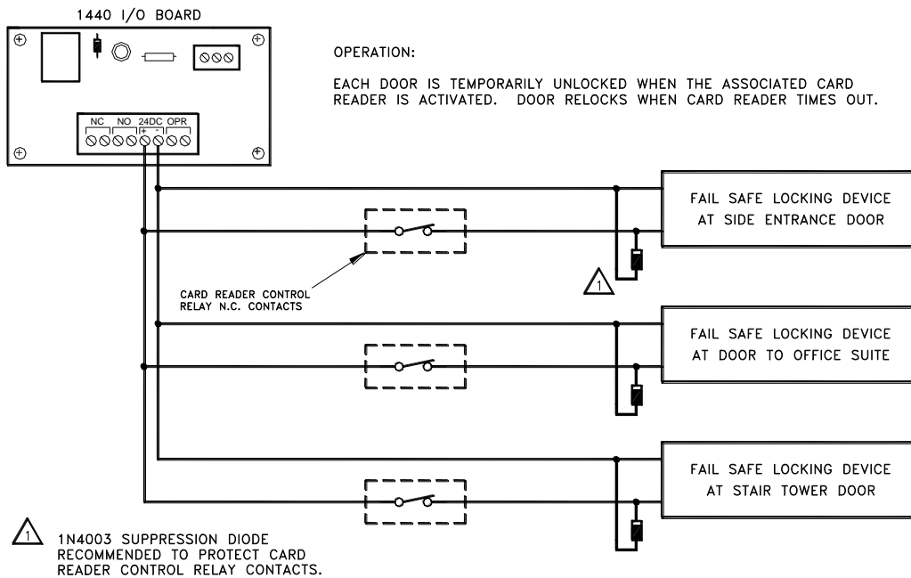
FIG. 4: WIRE SCHEME FOR INDEPENDENT CONTROL OF MULTIPLE DOORS
