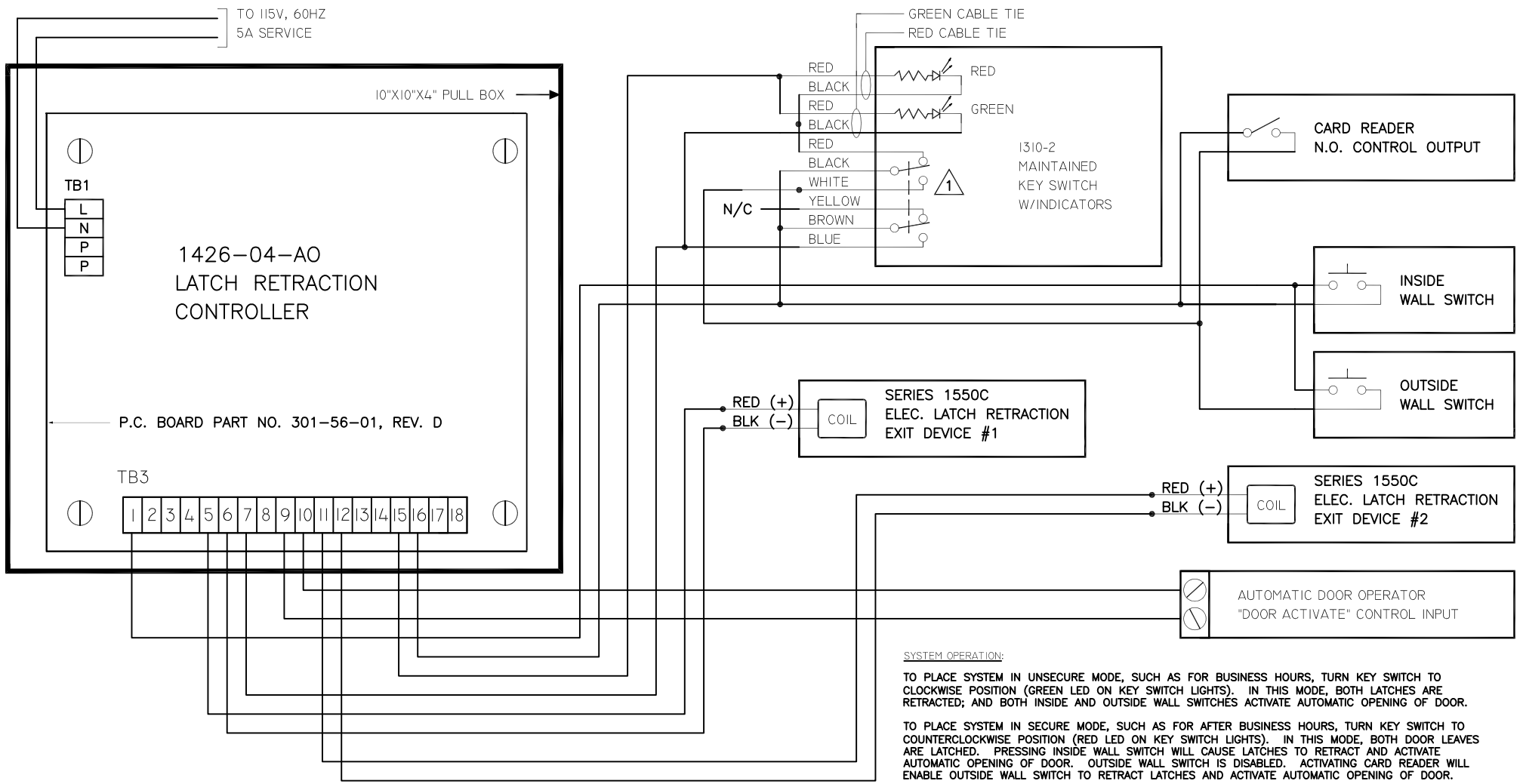
FIG. 5: POINT-TO-POINT FOR VARIATION 1 OF PAIR DOOR APPLICATION USING ACSI KEY SWITCH FOR SELECTING DAY/NIGHT MODE CONTROL
