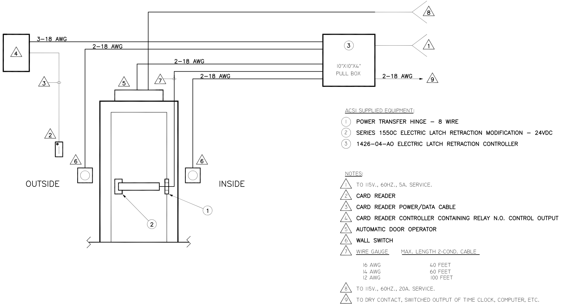
FIG. 4: TYPICAL RISER FOR SINGLE DOOR APPLICATION USING REMOTE OUTPUT (TIME CLOCK, COMPUTER, ETC.) FOR SELECTING DAY/NIGHT MODE CONTROL
