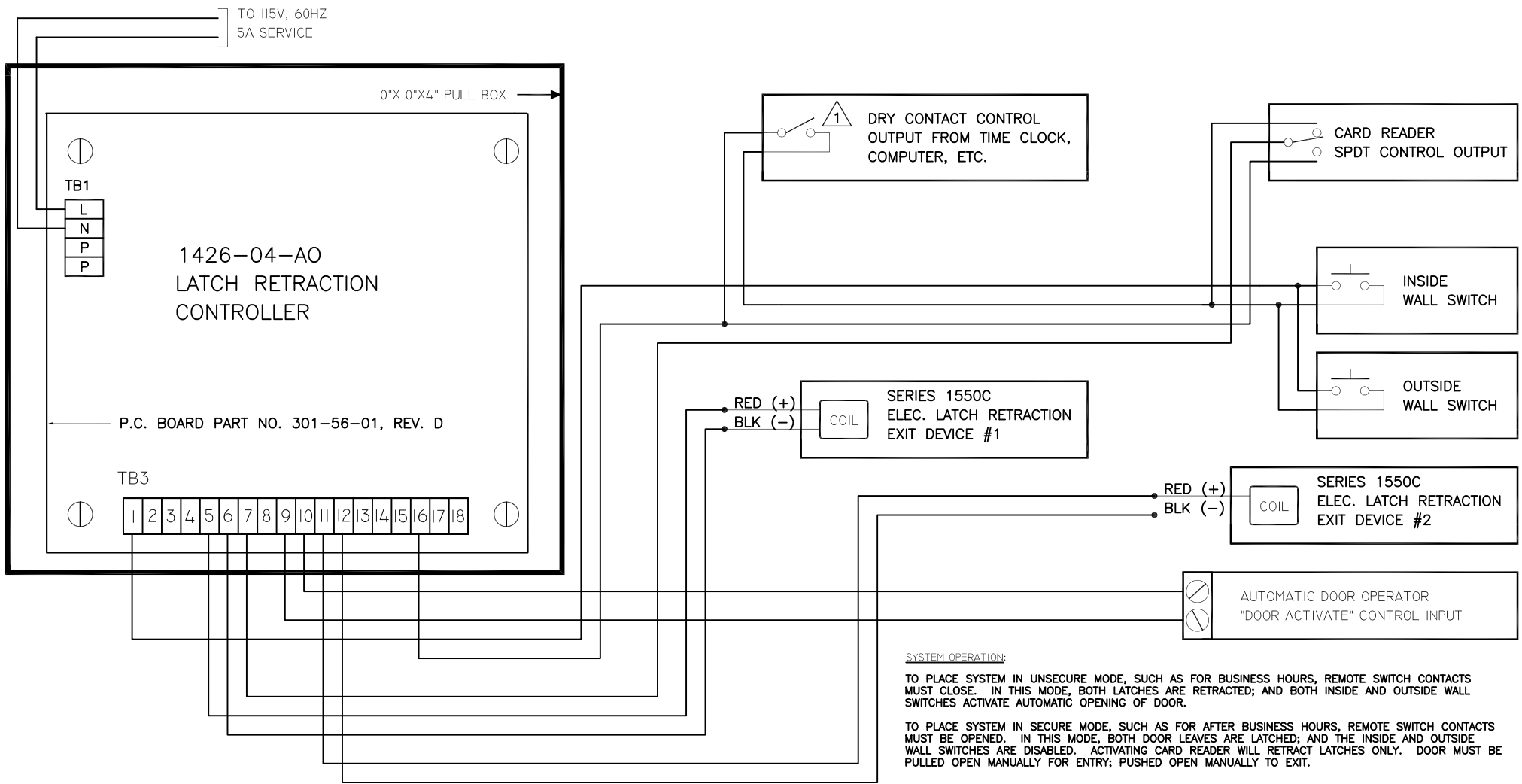
FIG. 12: POINT-TO-POINT FOR VARIATION 4 OF PAIR DOOR APPLICATION USING REMOTE OUTPUT (TIME CLOCK, COMPUTER, ETC.) FOR SELECTING DAY/NIGHT MODE CONTROL
