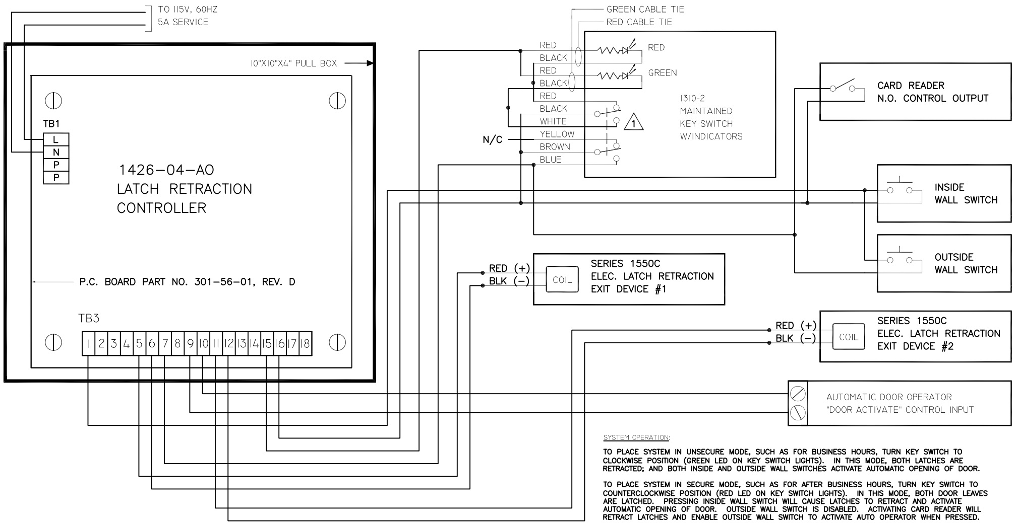
FIG. 6: POINT-TO-POINT FOR VARIATION 2 OF PAIR DOOR APPLICATION USING ACSI KEY SWITCH FOR SELECTING DAY/NIGHT MODE CONTROL
