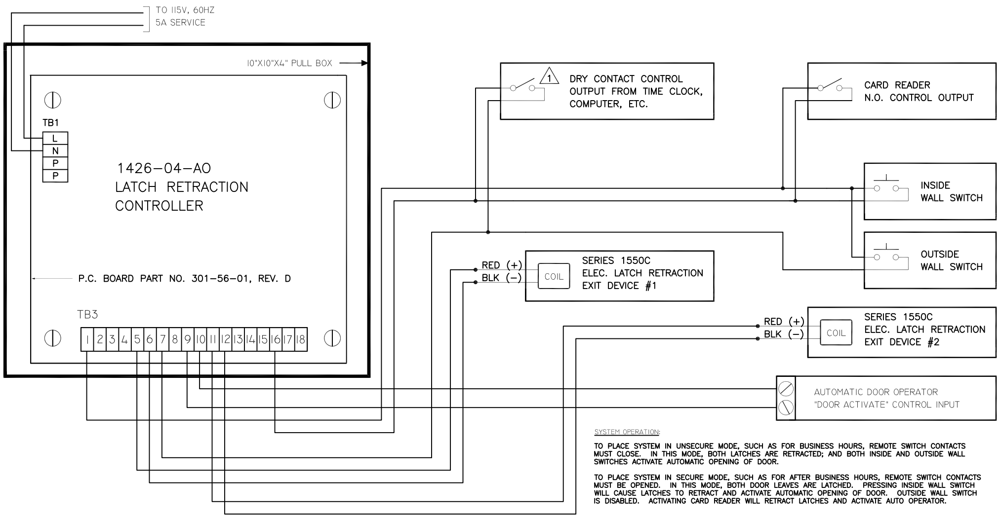
FIG. 11: POINT-TO-POINT FOR VARIATION 3 OF PAIR DOOR APPLICATION USING REMOTE OUTPUT (TIME CLOCK, COMPUTER, ETC.) FOR SELECTING DAY/NIGHT MODE CONTROL
