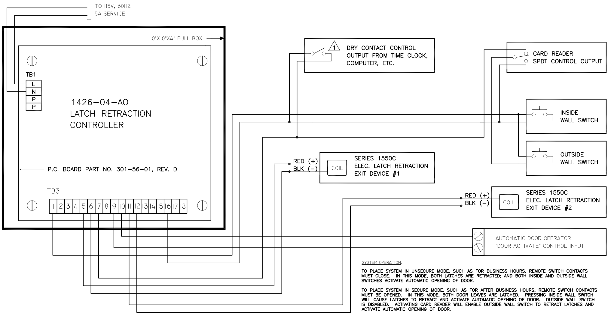
FIG. 9: POINT-TO-POINT FOR VARIATION 1 OF PAIR DOOR APPLICATION USING REMOTE OUTPUT (TIME CLOCK, COMPUTER, ETC.) FOR SELECTING DAY/NIGHT MODE CONTROL
