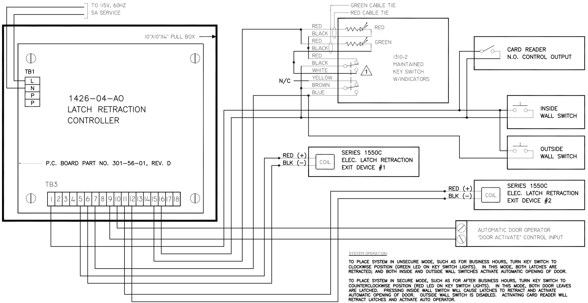
FIG. 7: POINT-TO-POINT FOR VARIATION 3 OF PAIR DOOR APPLICATION USING ACSI KEY SWITCH FOR SELECTING DAY/NIGHT MODE CONTROL
