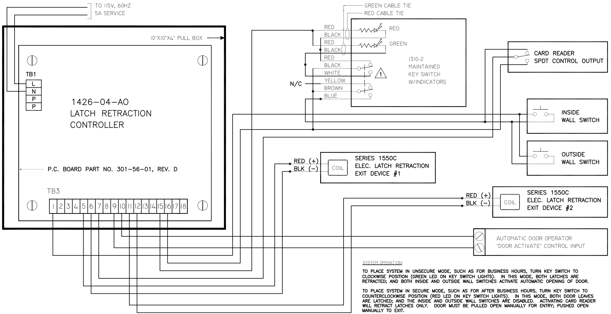
FIG. 8: POINT-TO-POINT FOR VARIATION 4 OF PAIR DOOR APPLICATION USING ACSI KEY SWITCH FOR SELECTING DAY/NIGHT MODE CONTROL
