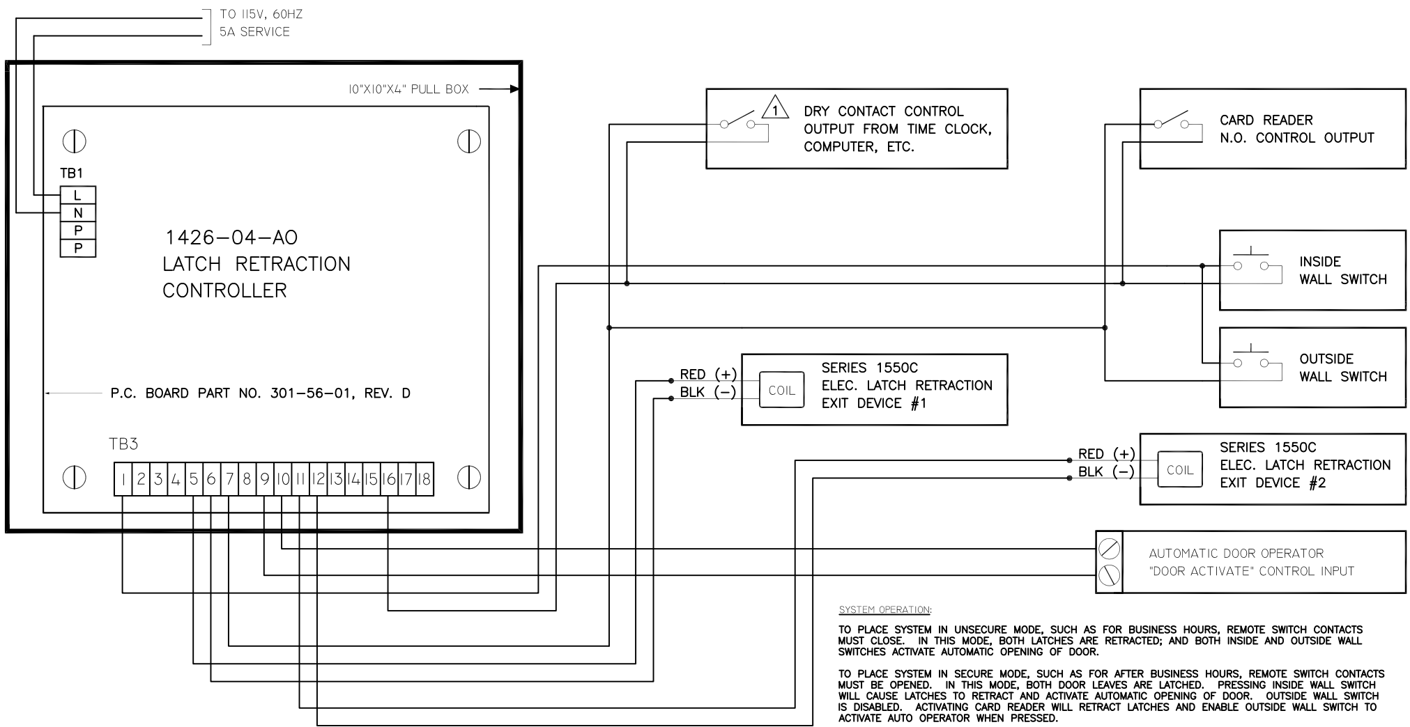
FIG. 10: POINT-TO-POINT FOR VARIATION 2 OF PAIR DOOR APPLICATION USING REMOTE OUTPUT (TIME CLOCK, COMPUTER, ETC.) FOR SELECTING DAY/NIGHT MODE CONTROL
