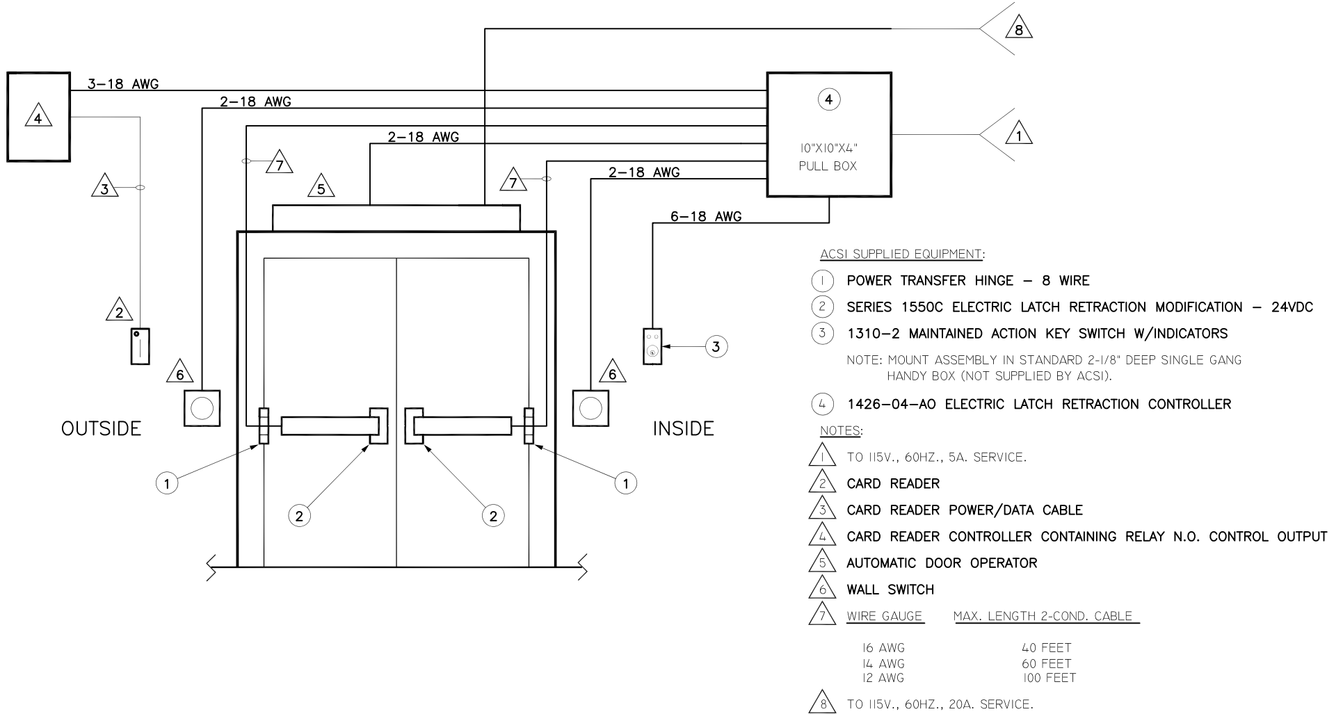
FIG. 1: TYPICAL RISER FOR PAIR DOOR APPLICATION USING ACSi KEY SWITCH FOR SELECTING DAY/NIGHT MODE CONTROL
