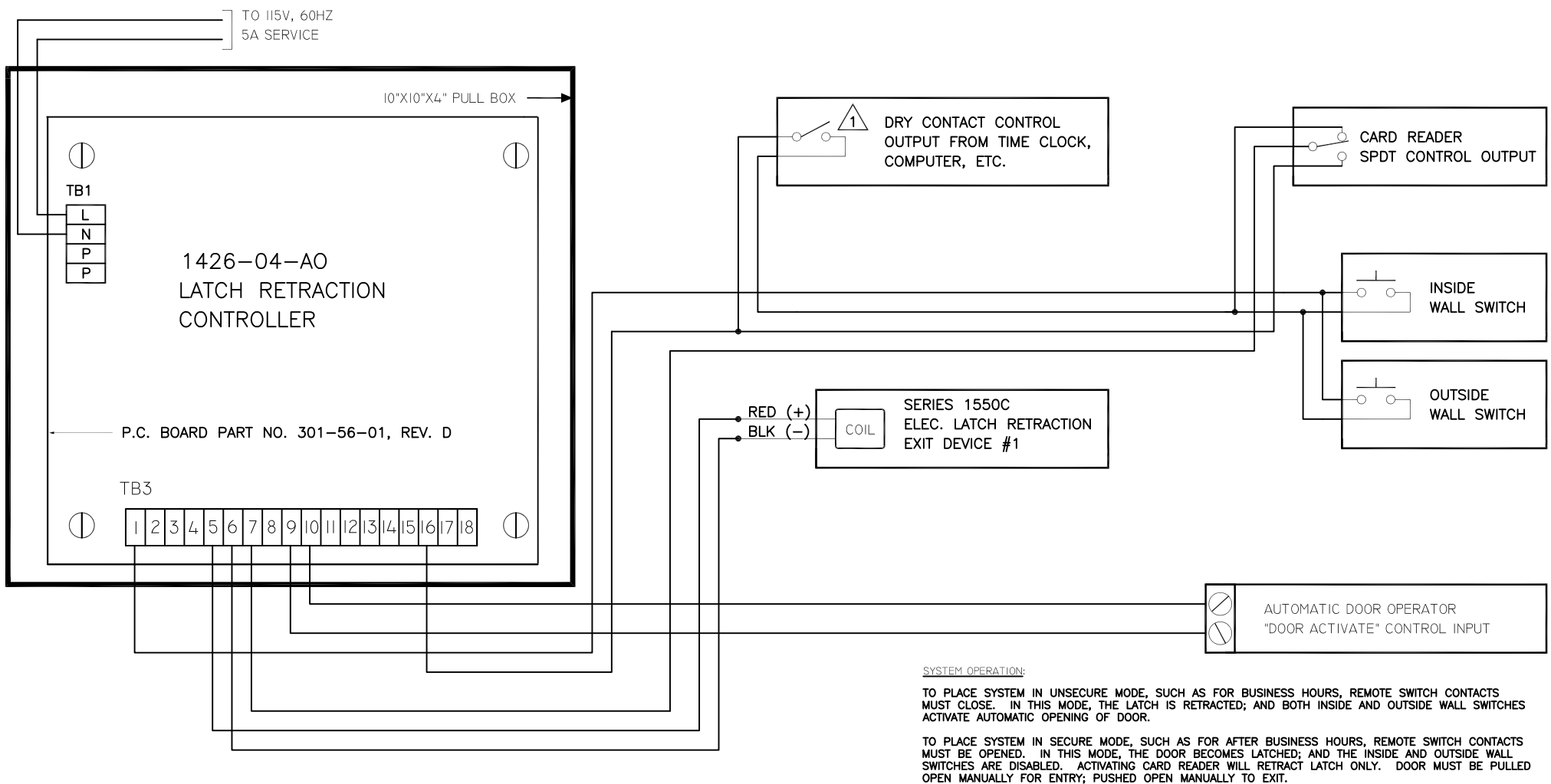
FIG. 20: POINT-TO-POINT FOR VARIATION 4 OF SINGLE DOOR APPLICATION USING REMOTE OUTPUT (TIME CLOCK, COMPUTER, ETC.) FOR SELECTING DAY/NIGHT MODE CONTROL
