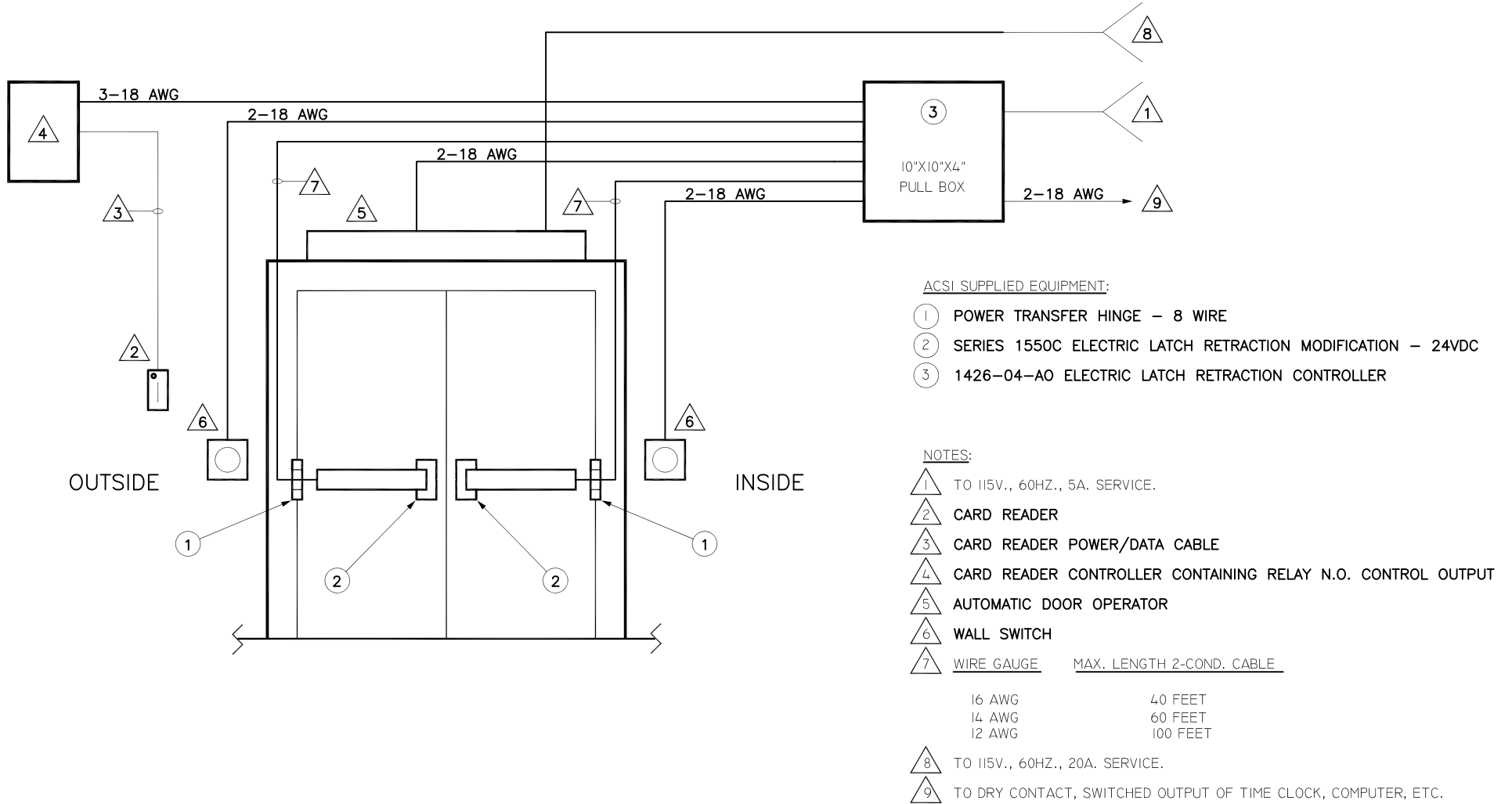
FIG. 2: TYPICAL RISER FOR PAIR DOOR APPLICATION USING REMOTE OUTPUT (TIME CLOCK, COMPUTER, ETC.) FOR SELECTING DAY/NIGHT MODE CONTROL
