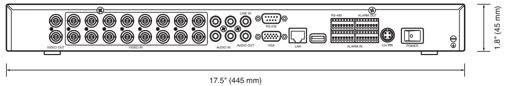
8/16-Channel DVR Rear View (16-channel DVR shown)
