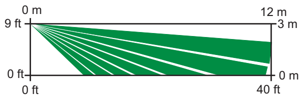
Side View Standard Broad Coverage: 12 m x 12 m (40 ft x 40 ft)
