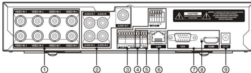
Figure 2: 8-Channel DVR rear panel.
