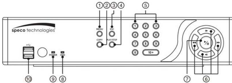
Figure 3: 8-Channel DVR front panel.
