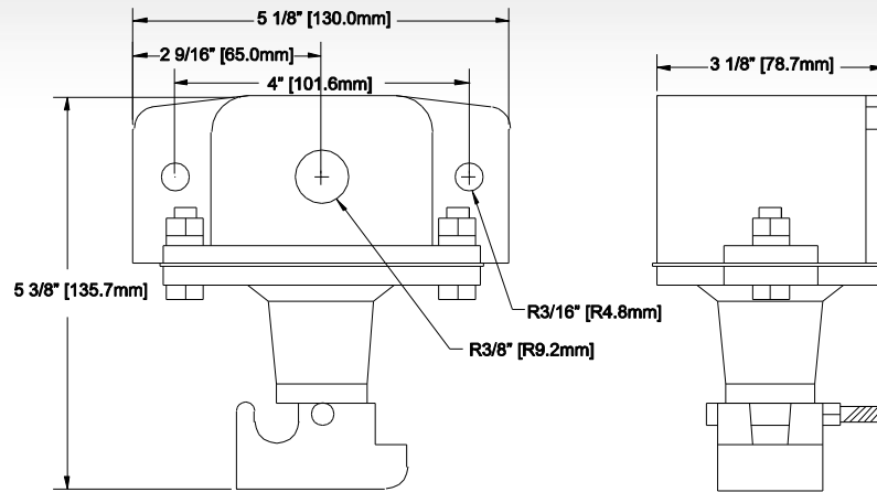
Figure 5 - CI-WPS1 Mechanical
