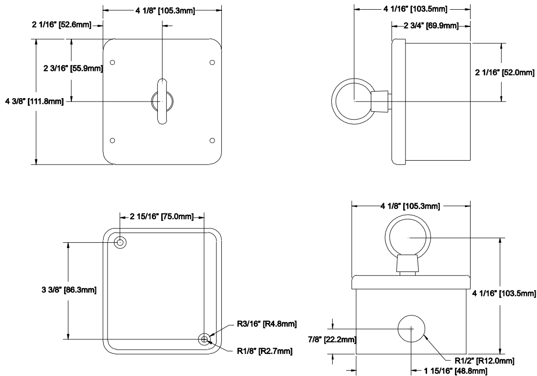
Figure 6 - CI-SCP1 Mechanical
