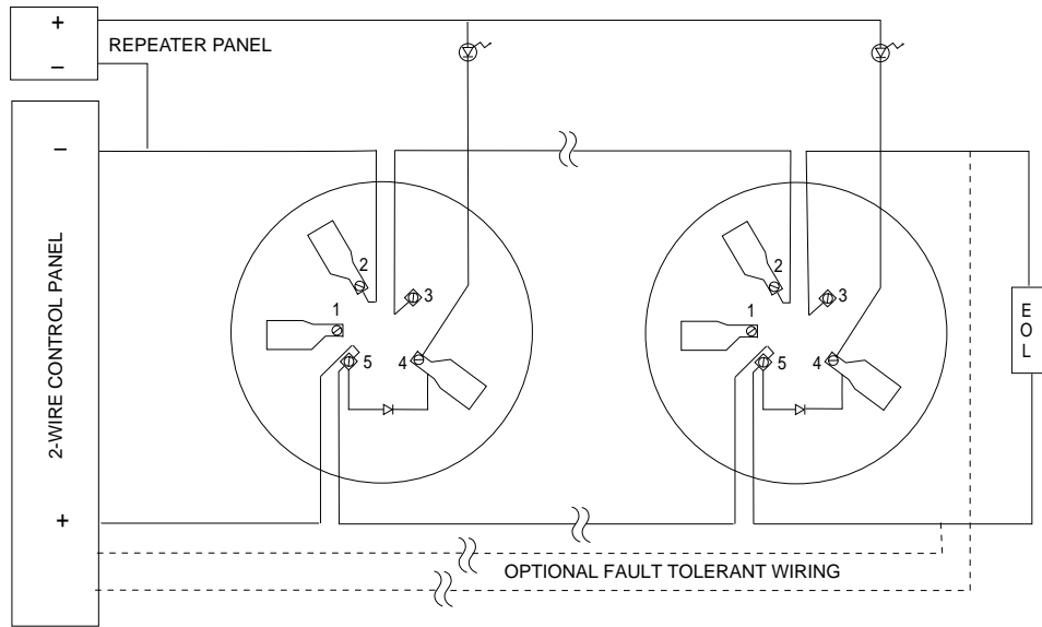
Figure 2. Typical wiring diagram for 2-wire detector systems:
