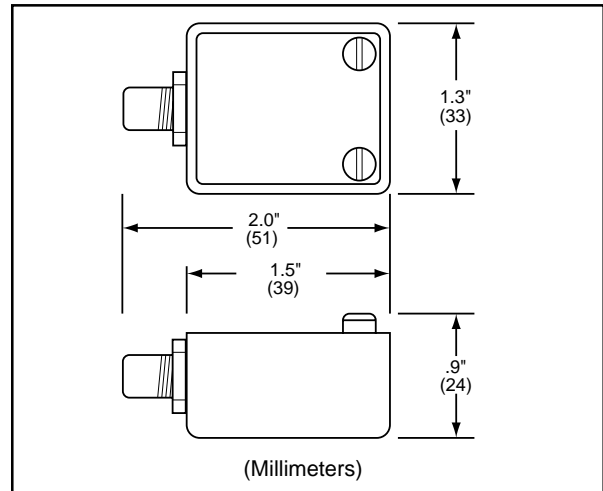
AS1000 Drawing
