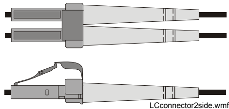
Figure 3 LC Connector
