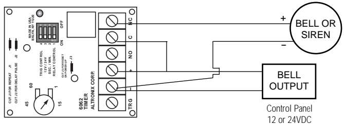
Fig. 7 - Bell Cut Off Timer:
