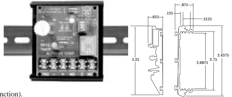
ST3 Mechanical Drawing
