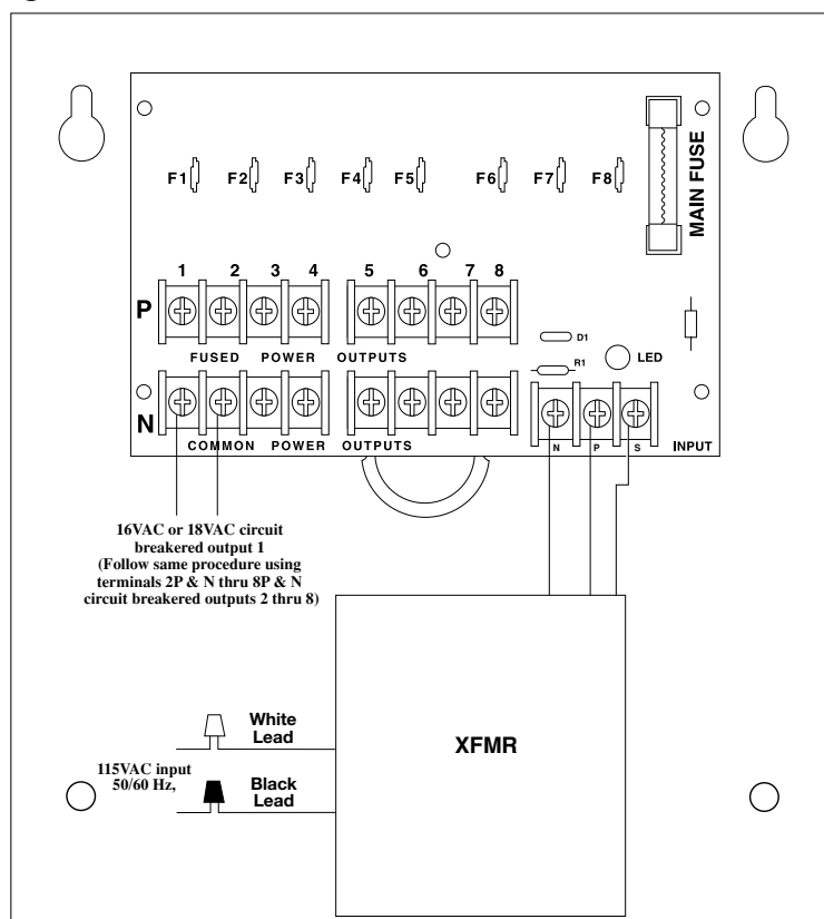
Back Panel of Enclosure
