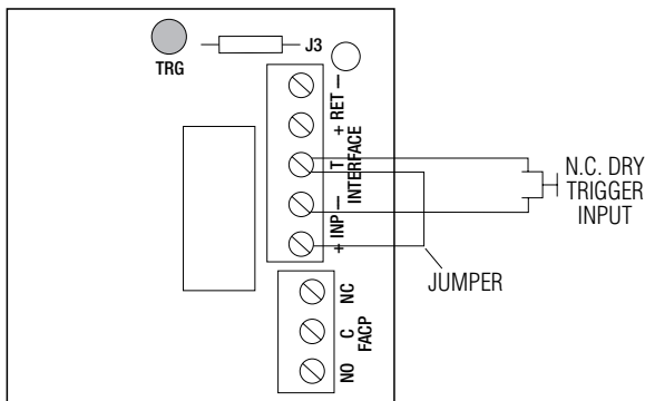
Fig. 6 Normally Closed - Non-Latching FACP trigger input:
