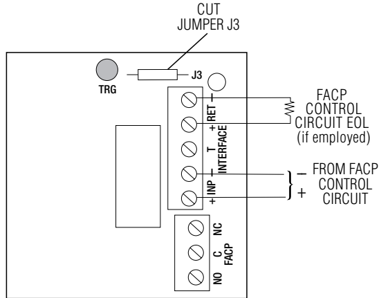
Fig. 3 Polarity reversal input from FACP signaling circuit output (polarity is referenced in alarm condition): (This output has not been evaluated by UL)
