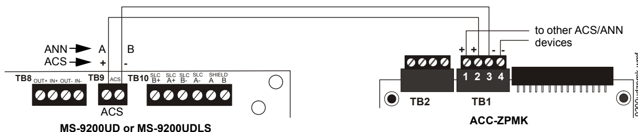
Figure D.2 Connection for MS-9200UD or MS-9200UDLS to ACC-ZPMK
