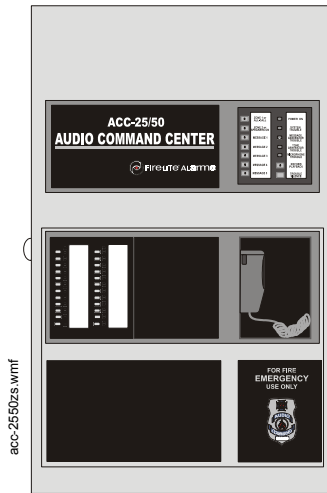
Figure 3.1 ACC-25/50ZS Cabinet
