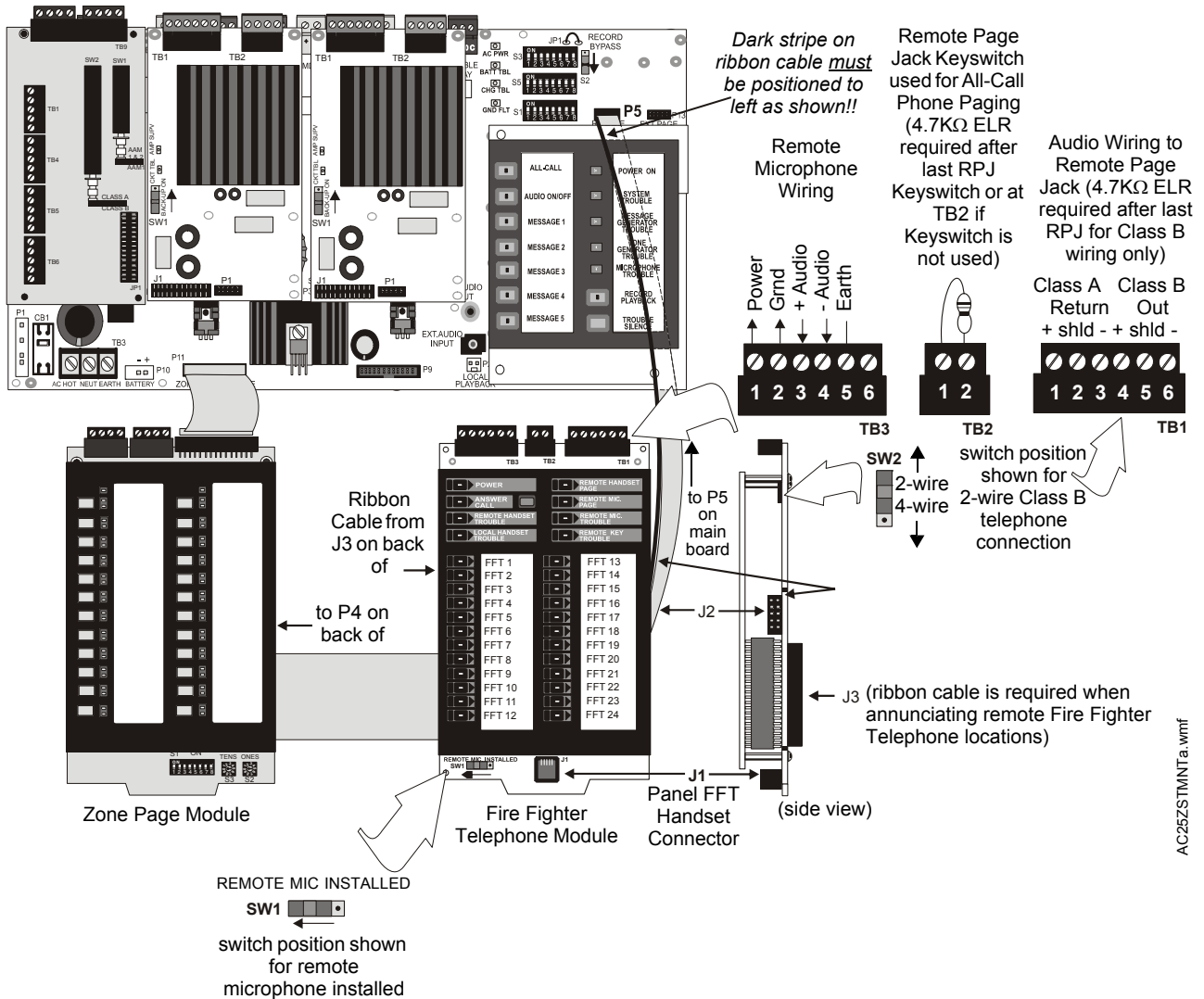
Figure 1.4 ACC-25/50ZST Main Board with ACC-FFT Module
