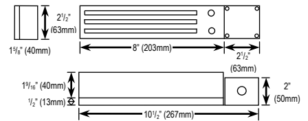
Magnetic Lock and Bracket
