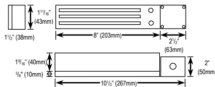
Magnetic Lock and Bracket
