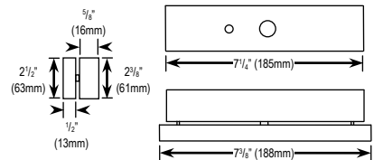
Armature Plate and Bracket
