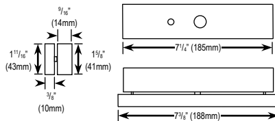
Armature Plate and Bracket
