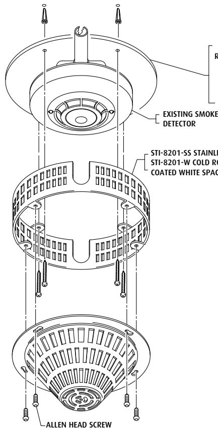
SURFACE MOUNT INSTALLATION
