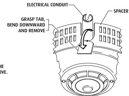
VIEW SHOWING SPACER INSTALLATION WITH CONDUIT ENTRY
