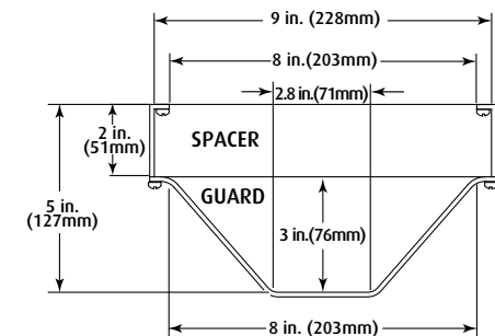
PRODUCT DIMENSIONS
