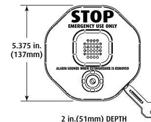
PRODUCT DIMENSIONS
