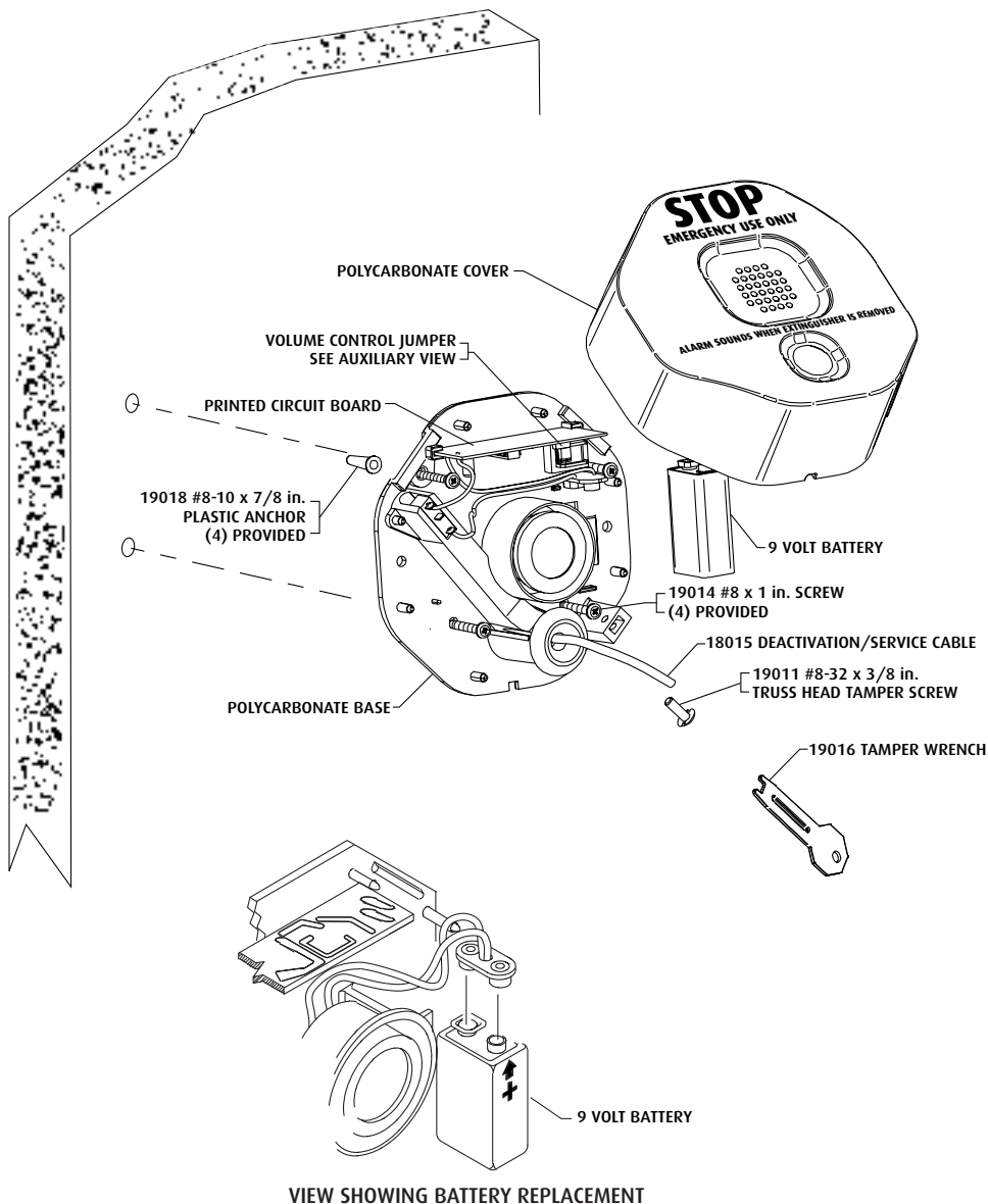
VIEW SHOWING BATTERY REPLACEMENT
