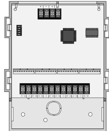
5880 IO / LED Driver Module
