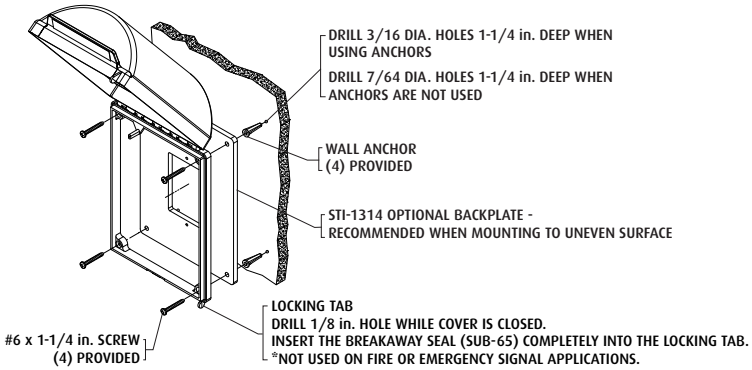
Fig. 3 - Surface Mounting Option - Models 132** & 142**
