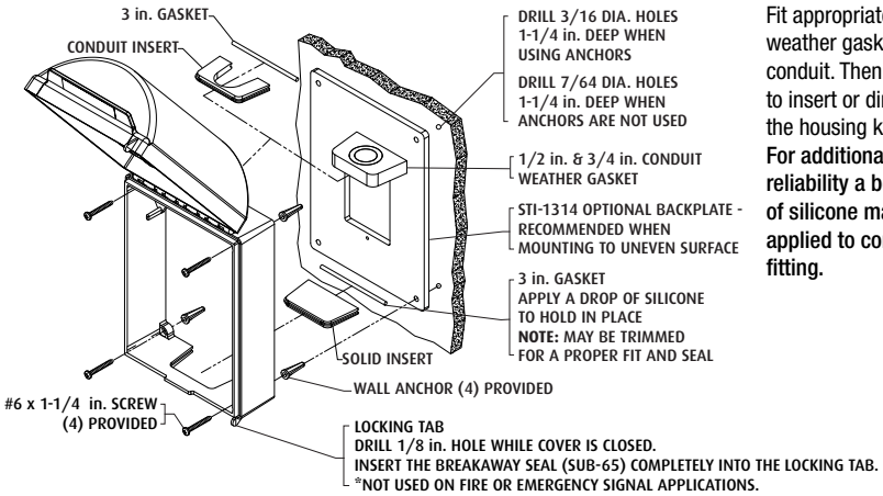
Fig. 4 - Enclosed Flush Mounting Option - Models 133** & 143** NEMA TYPE 3RX
