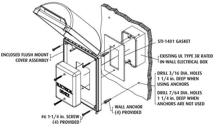
Fig. 4 - Enclosed Flush Mounting Option - Models 133** & 143** NEMA TYPE 3RX
