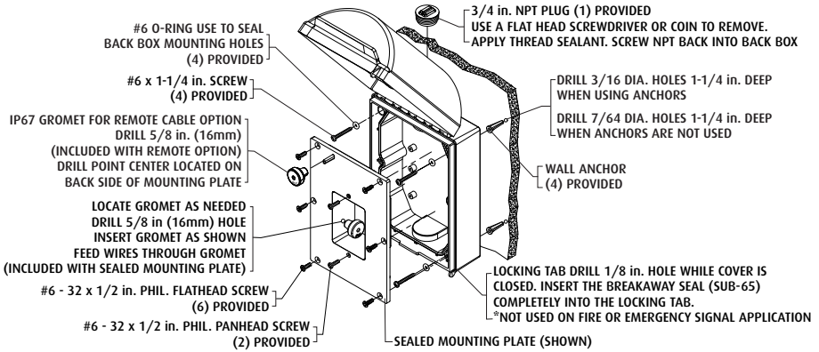
Fig. 5 - Enclosed Back Box Mounting Option - Models 134**, 135**, 138**, 139**, 144**, 145**, 148** & 149** NEMA TYPE 3RX
